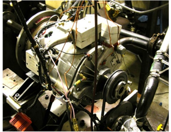
RotaPower LLC 530cc Compound Rotary Engine on Dynamometer
